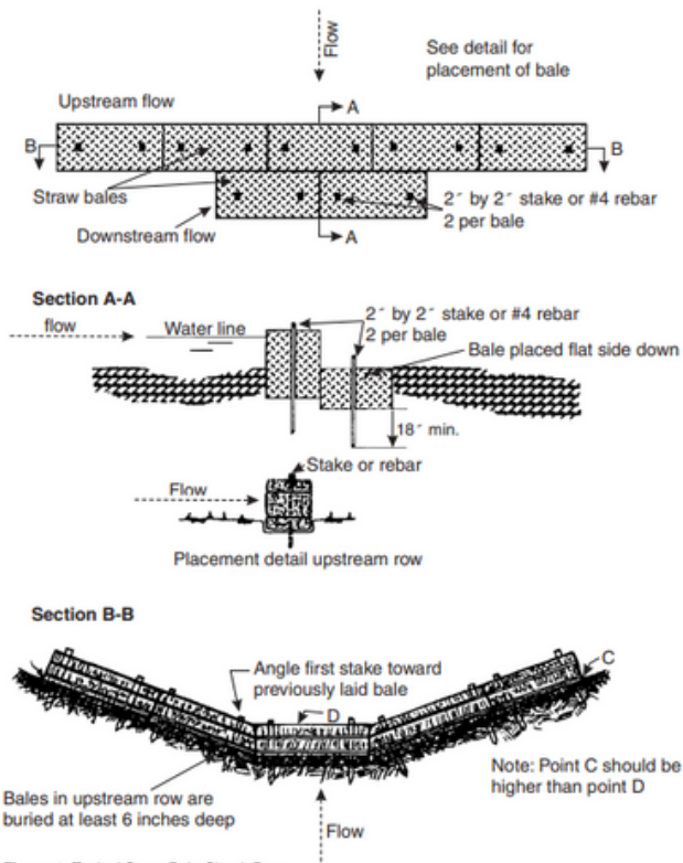
Figure 4: Typical Straw Bale Check Dam
